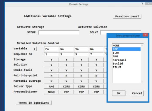
Selection of Preconditioners
