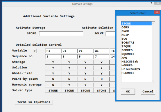
Selection of Solvers
