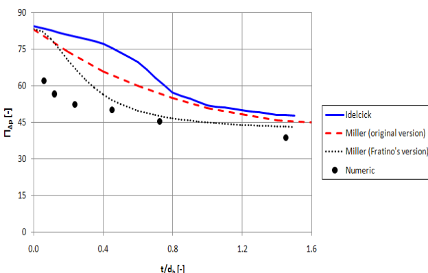
Figure 4 Trend of the pressure drop coefficient \Pi_{\Delta p} as a function of the relative thickness t/d_h for the plate shown in Figure 1 ( \beta=0.39 ): comparison among numerical predictions and literature models for the single-hole case.
