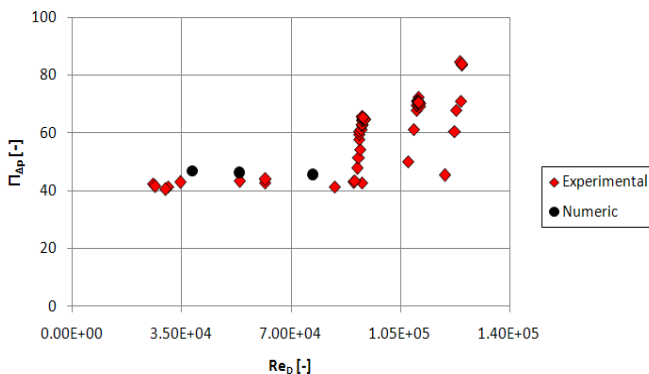
Figure 3 Trend of the pressure drop coefficient \Pi_{\Delta p} as a function of the pipe Reynolds number Re_D for the plate shown in Figure 1 ( \beta=0.39 ) with t/d_h=0.73 : comparison among experimental data and numerical predictions.
