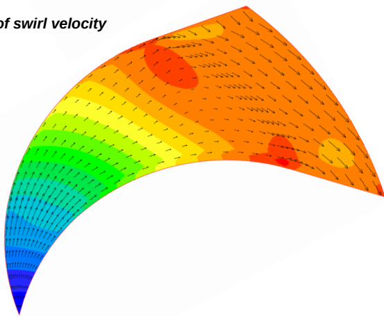
Pressure and swirl velocity contours from 3-D rotor analysis
