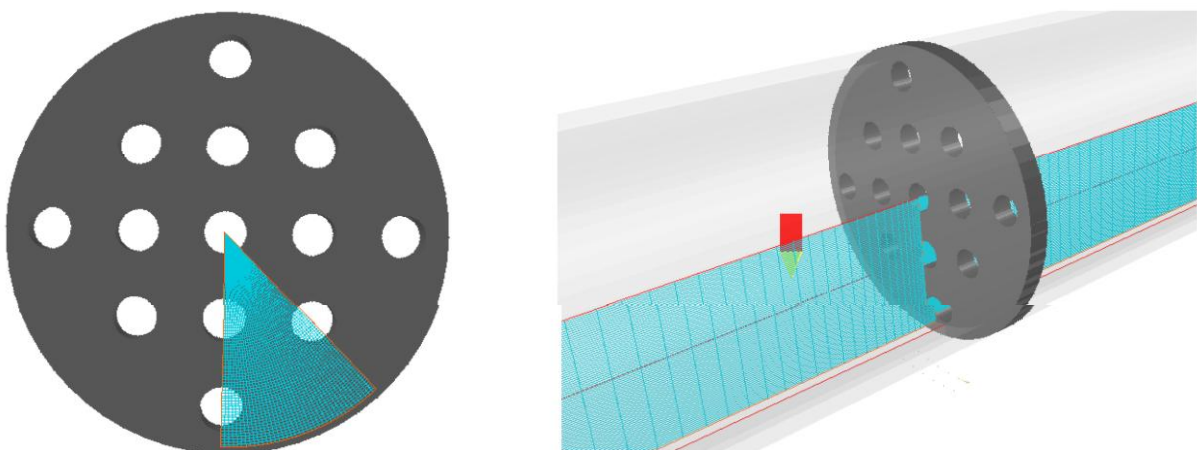
Figure 2 The cylindrical-polar mesh used in the simulations: planar view (left) and side view (right).
