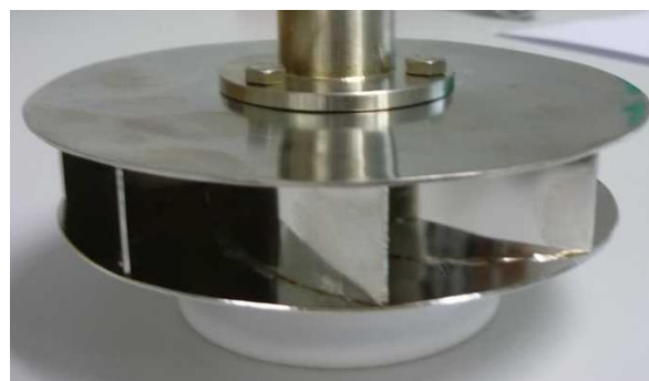
Picture of a typical “induced-draft rotor” used for foam separation
