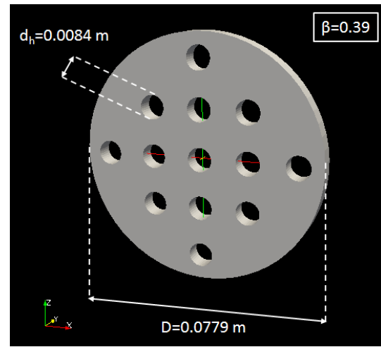
Figure 1 The plate considered in the simulations.
