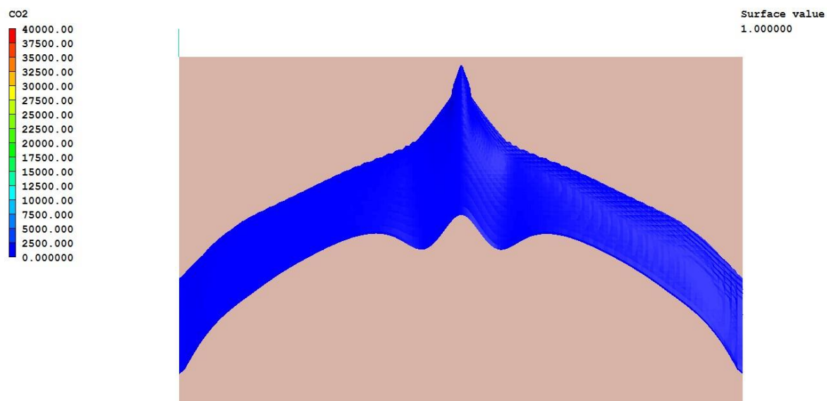
Figure 15: Iso-surface of \text{CO}_2 concentration at 1 ppm
