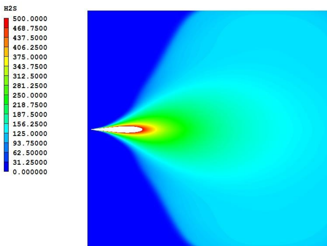
Figure 9: H 2 S concentration in ppm –Top view (Zoomed)
