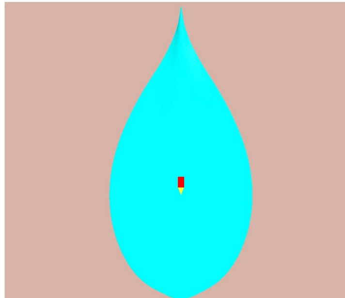
Figure 21: a) H_2S dispersion in the x direction. The red line highlights the 130 ppm concentration. These data are taken at 1070m from the pipeline indicated by the probe position in b); b) H_2S isosurface 130 ppm dispersion in the x direction
