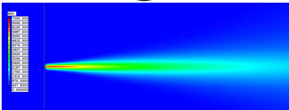
Figure 9: H 2 S concentration in ppm –Top view (Zoomed)
