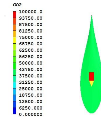
Figure 18: a) CO 2 dispersion in the x direction. The red line highlights the 40000 ppm concentration. These data are taken at 470m from the pipeline indicated by the probe position in b); b) CO 2 isosurface 40000ppm
