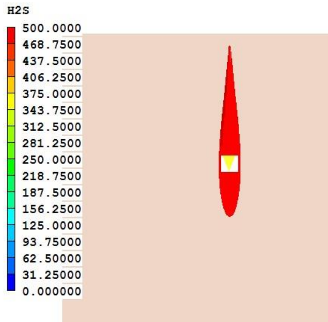
Figure 19: a) H_2S dispersion in the x direction. The red line highlights the 500 ppm concentration. These data are taken at 270m from the pipeline indicated by the probe position in b); b) H_2S isosurface 500 ppm dispersion in the x direction.
