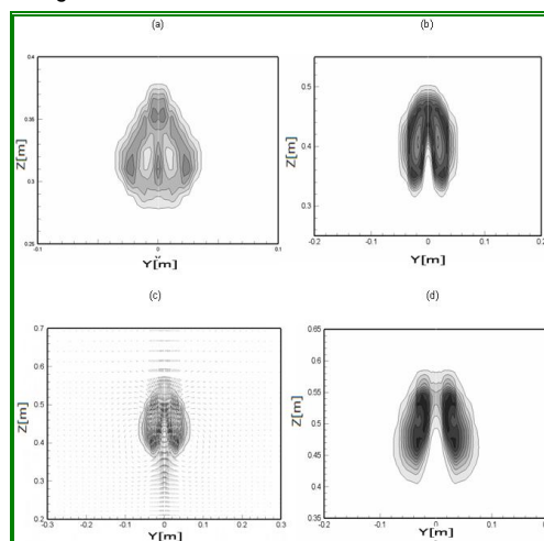
Figure 2. Mean shape for V_f/V_x=0.5 at four different downstream locations of the stack: a) x/D=3.5 , b) x/D=17 , c) x/D=21 y d) x/D=26 . Flame borders are defined by means of heat radiation contours. V_f is the propane discharge velocity, V_x corresponds to the cross flow velocity and D is the diameter of the stack.
