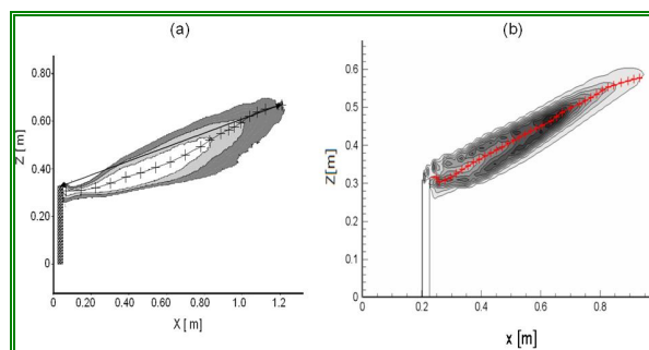
Figure 1. Mean flame trajectory for a cross flow velocity V_x of 2.0 m/s, ( V_f/V_x=0.5 ), a) Experimental data (Majeski, et al. 1999) and b) Numerical results (flame borders are defined by means of heat radiation contours). V_f is the propane discharge velocity and V_x corresponds to the cross flow velocity.
