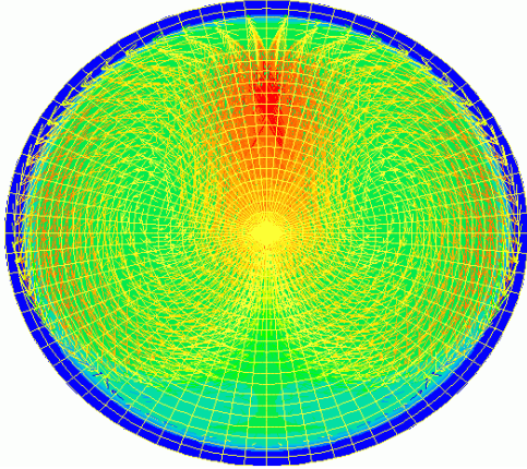
Velocity vectors & temperature contours in cooled tubes influenced by gravity acting in the vertical direction.
