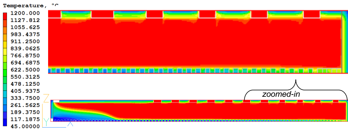
Figure 2 – Temperature distribution after 62.5 minutes
