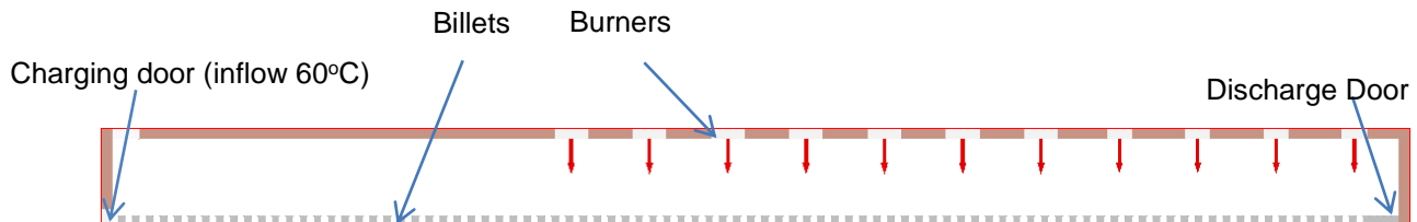
Figure 1 – 2D transient CFD model showing charging door, discharge door, billets and burners
