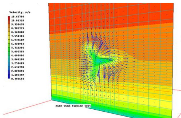
Figure 3. Velocity magnitude contour plot in the plane of a modelled turbine with superimposed in-plane velocity vectors.
