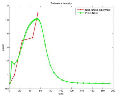
Figure 5. Comparison of PHOENICS results for the turbulence intensity with experimental results from the Nibe wind turbine experiments. The surface roughness is assumed to be 0.08m and the friction velocity 0.46m/s.
