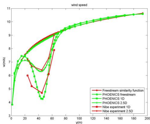
Figure 4. Comparison of PHOENICS results for the axial wind velocity with experimental results from the Nibe wind turbine experiments. The surface roughness is assumed to be 0.08m and the friction velocity 0.56m/s.
