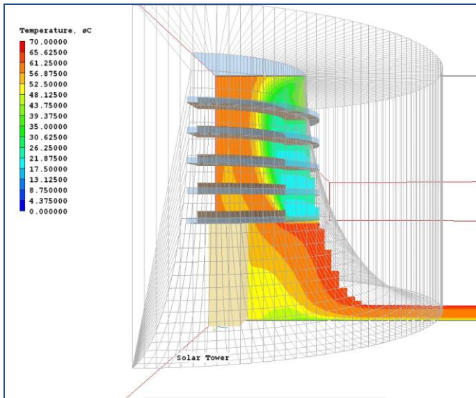
Temperature contours
