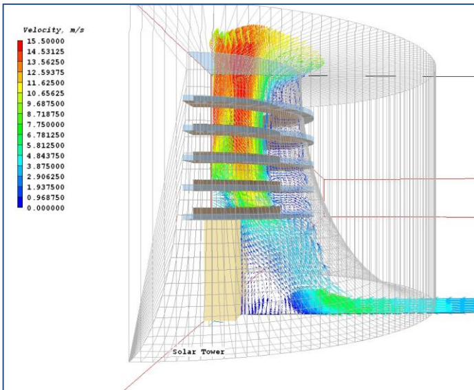
Velocity vectors
