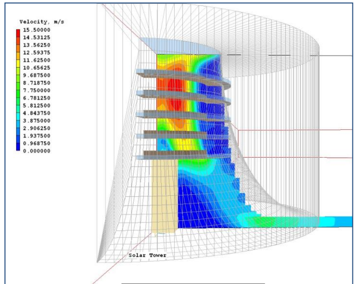
Velocity contours
