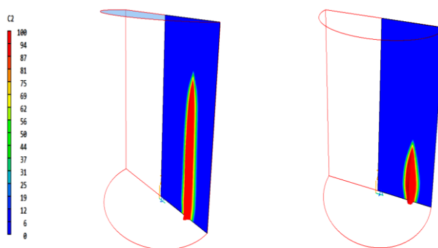
Figure 1: Single-plug Design: Contour plots of C2 scalar (tracer) concentration along plane of injection at 0.5 s. This also shows the 90% tracer iso-surface. Case A, left and case B, right.
