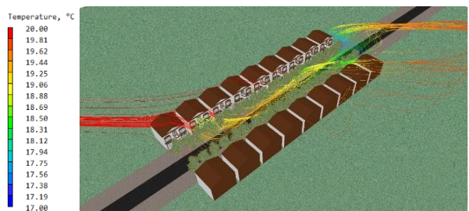
Figure 3: Streamline plot, coloured by temperature, showing the origin and destination of flow along the centre of the street at pedestrian level. Scale: Red – 20^\circ\text{C} ; Blue – 17^\circ\text{C}
