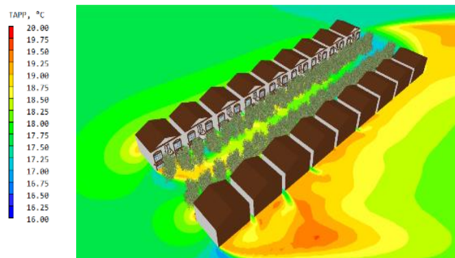
Figure 6: Contour plot of apparent temperature at pedestrian level showing up to 3 °C of cooling towards the leeward end of the street. Scale: Red – 20 °C; Blue – 16 °C
